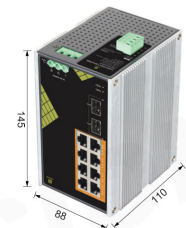
Dimension (mm)
